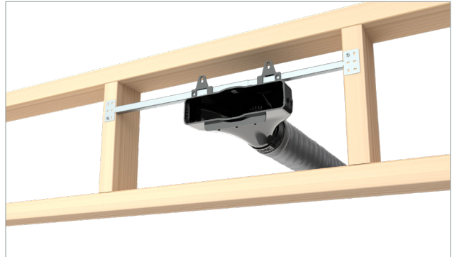
Pass Through Boot Assembly installed with Hanger Bar
