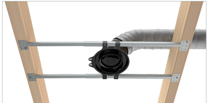
Ceiling Boot Assembly installed with two Hanger Bars
